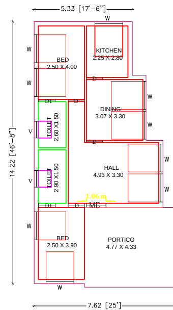
GROUND FLOOR PLAN EAST FACING
