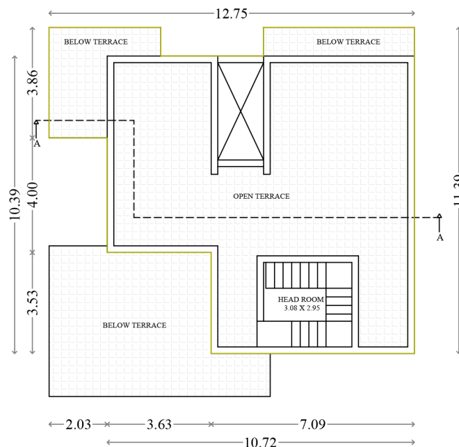
TERRACE FLOOR
