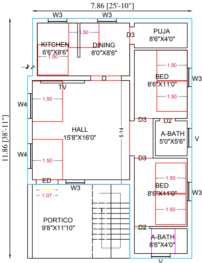
PROPOSED GROUND FLOOR PLAN (NORTH FACING)
