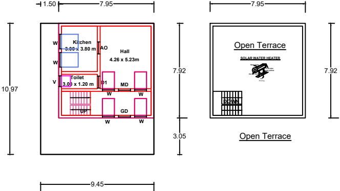
Ground Floor Plan (East Facing)
