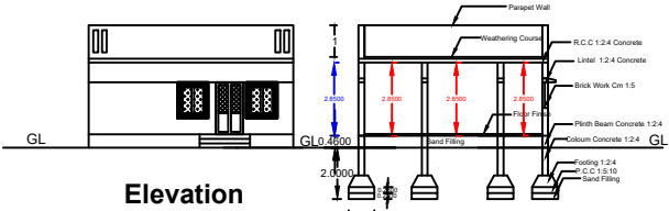
Section Section - AA
