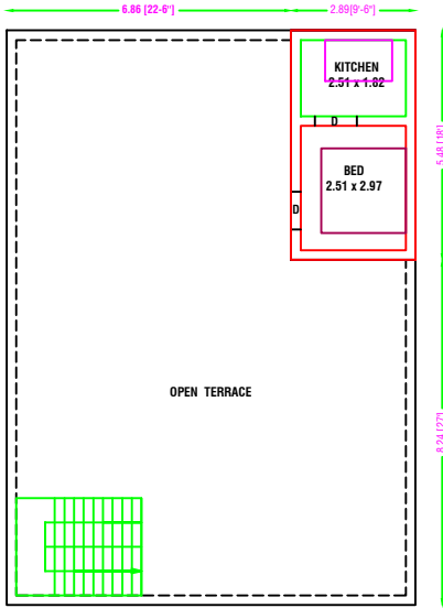
PRO. FIRST FLOOR PLAN [ WEST FACING]
