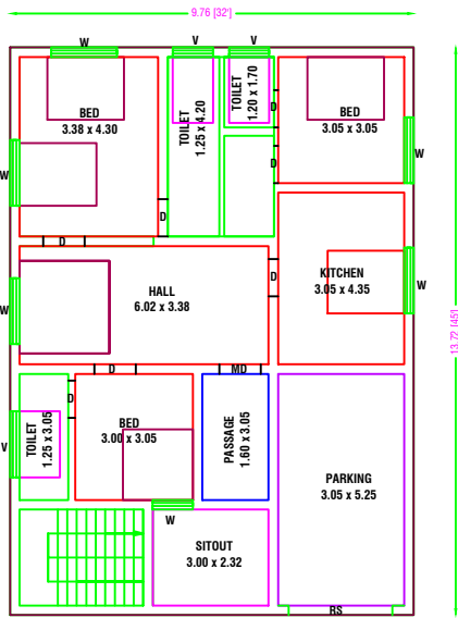
PRO. GROUND FLOOR PLAN [ WEST FACING]
