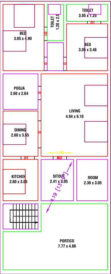
GROUND FLOOR PLAN [EAST FACING]
