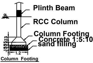
Foundation Detail
