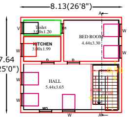
EX.GROUND/FLOOR PLAN ( NORTH FACING)
