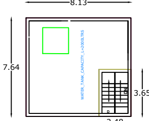
TERRACE FLOOR PLAN
