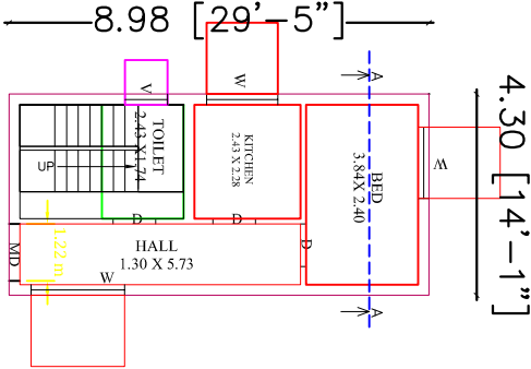
GROUND FLOOR PLAN (EAST FACING)
