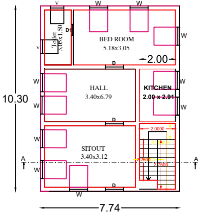
GROUND FLOOR PLAN ( SOUTH FACING)
