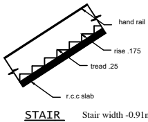
STAIR Stair width -0.91m
