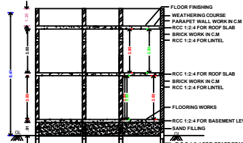
SECTION ON "BB"
