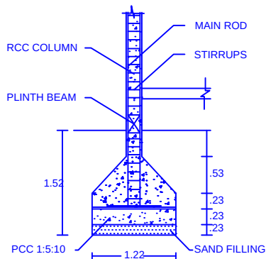
COLUMN DETAILS
