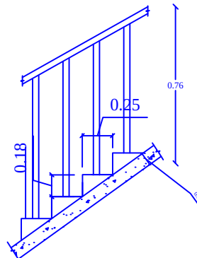
SECTION OF STAIRCASE
