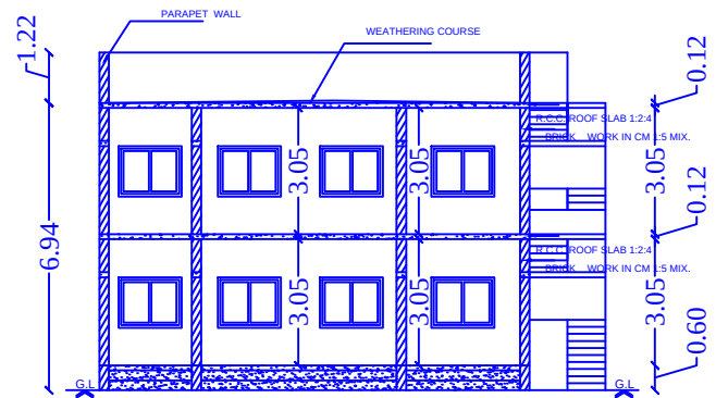
Section on-"AA"
