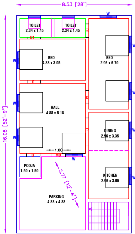
GROUND FLOOR PLAN [SOUTH FACING]
