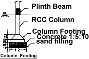
Foundation Detail
