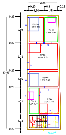
PROPOSED GROUND FLOOR PLAN
