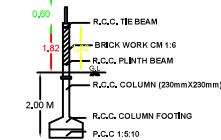
COMPOUND WALL DETAILS
