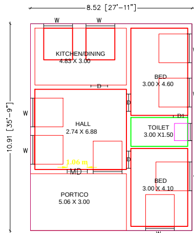
GROUND FLOOR PLAN NORTH FACING
