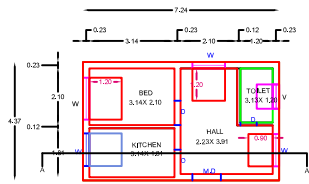
PROPOSED GROUND FLOOR PLAN (EAST FACING)
