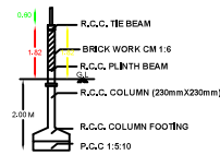
COMPOUND WALL DETAILS
