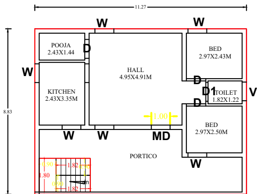
EXIS GROUND FLOOR PLAN
