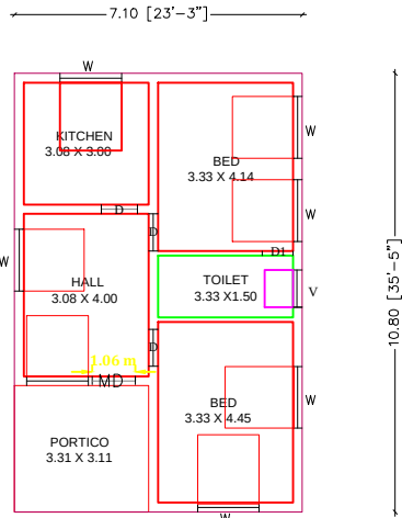
GROUND FLOOR PLAN NORTH FACING
