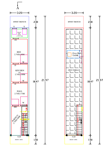
OPEN TERRACE PLAN
