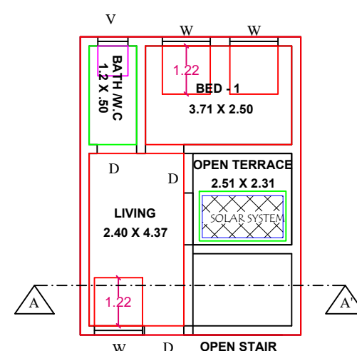
FIRST FLOOR PLAN - EAST FACING
