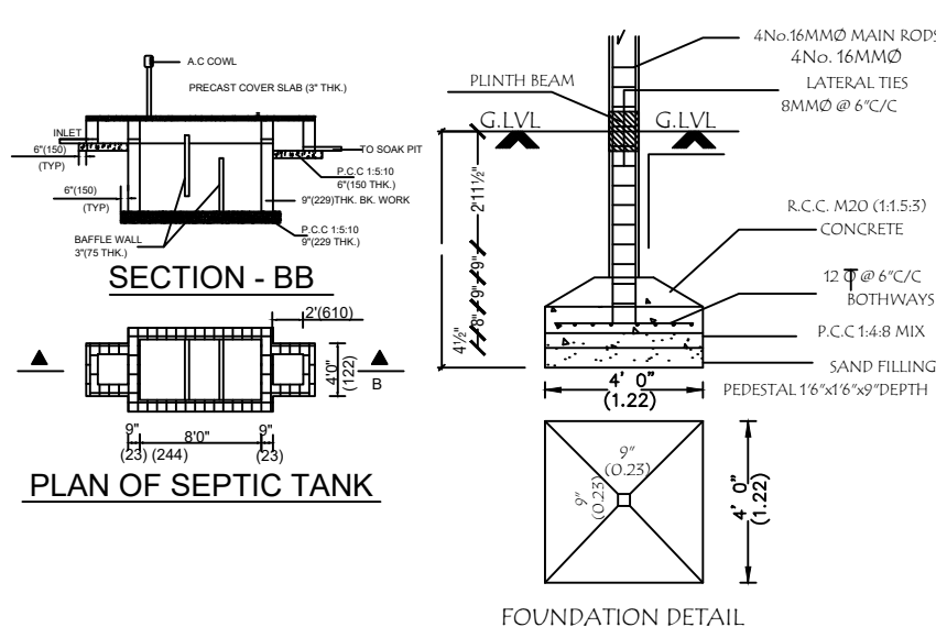
FOUNDATION DETAIL
