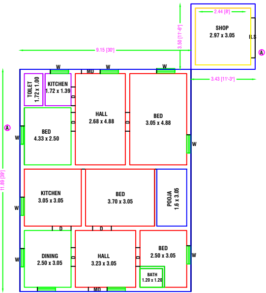
EX. GROUND FLOOR PLAN [ NORTH FACING ]
