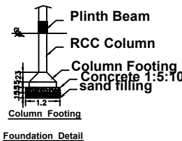
Column Footing
