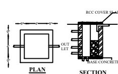
RAIN WATER COLLECTION PIT DETAILS
