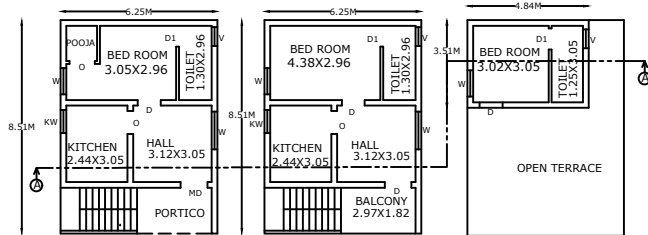
GROUND FLOOR PLAN SCALE - 1 : 100
