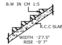
STAIR DETAILS
