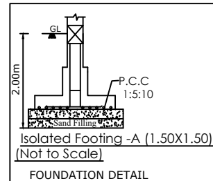
FOUNDATION DETAIL
