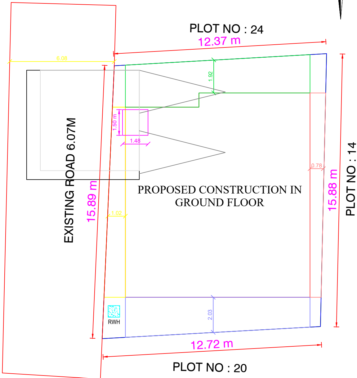
SITE PLAN
