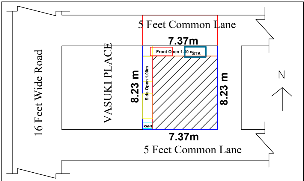
SITE PLAN
