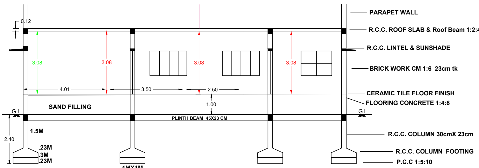
SECTION ON X-X' AXIS
