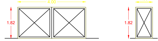
WICKET GATE
