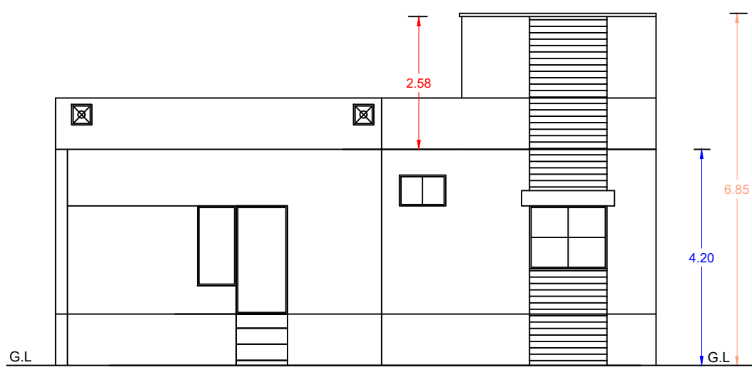
FRONT ELEVATION
