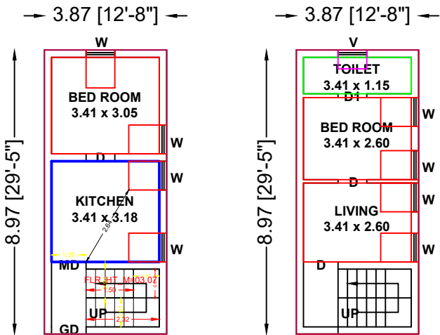
GROUND FLOOR PLAN (SOUTH FACING)
