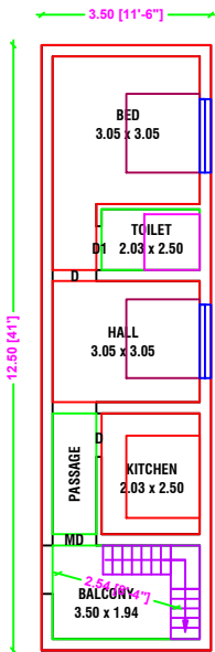
PRO.FIRST FLOOR PLAN WEST FACING
