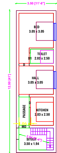
PRO.GROUND FLOOR PLAN WEST FACING
