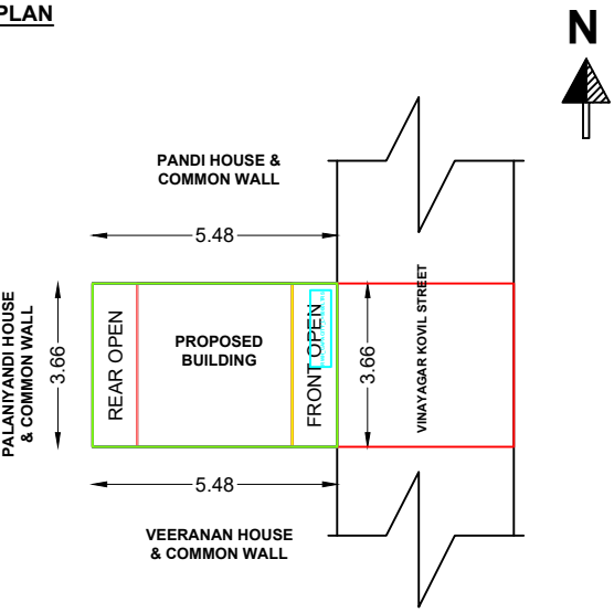
SITE PLAN
