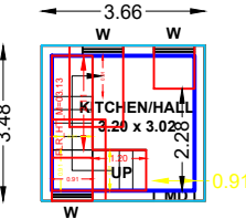
GROUND FLOOR PLAN (EAST FACING)
