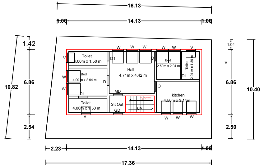
EXISTING GROUND FLOOR PLAN SOUTH FACING
