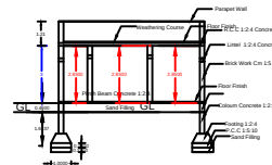
Section Section - AA
