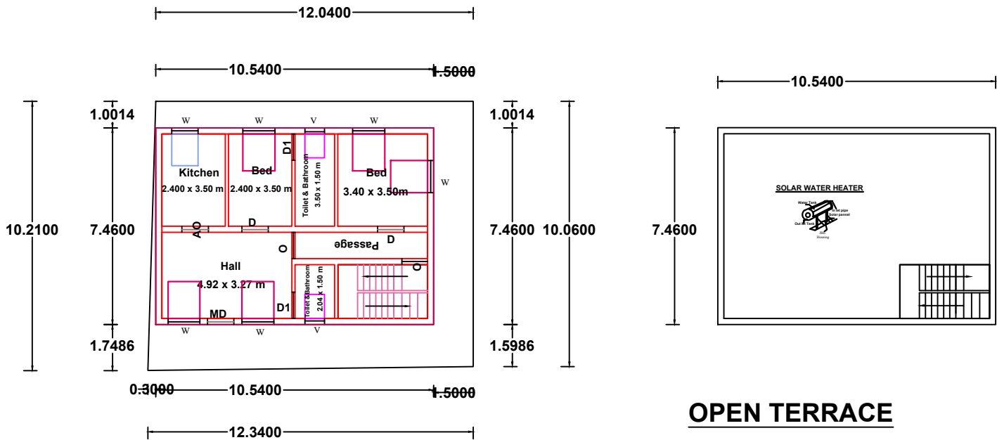
GROUND FLOOR PLAN (NORTH FACING )
