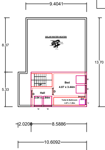
FIRST FLOOR PLAN & OPEN TERRACE
