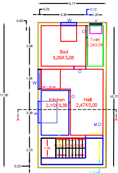
PROPOSED GROUND FLOOR PLAN (EAST FACING)
