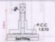
Isolated Footing - A (1.50X1.50) (Not to Scale)
