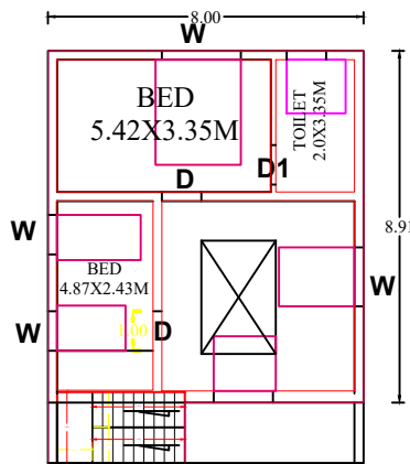
PRO FIRST FLOOR PLAN
