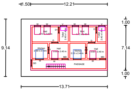
GROUND FLOOR PLAN (EAST FACING)
