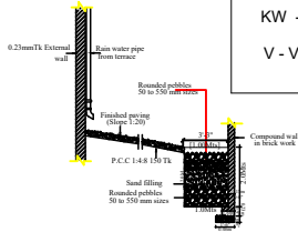
PLAN OF RAIN WATER HARVESTING
