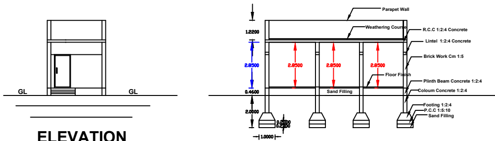
Section Section - AA
