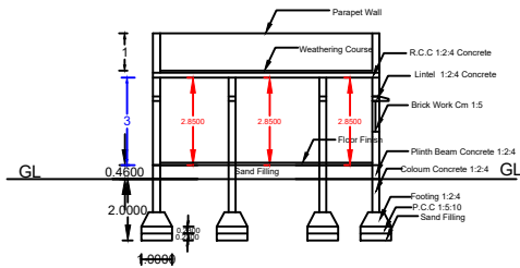
Section Section - AA
