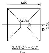
SECTION - 'CD'
