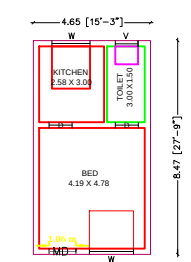
GROUND FLOOR PLAN SOUTH FACING
