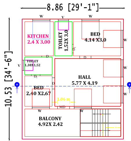
FIRST FLOOR PLAN (NORTH FACING)
