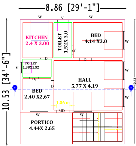
GROUND FLOOR PLAN (NORTH FACING)
