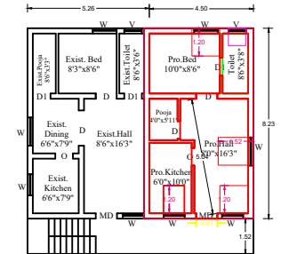
EXISTING AND EXTENSION OF GROUND FLOOR PLAN
