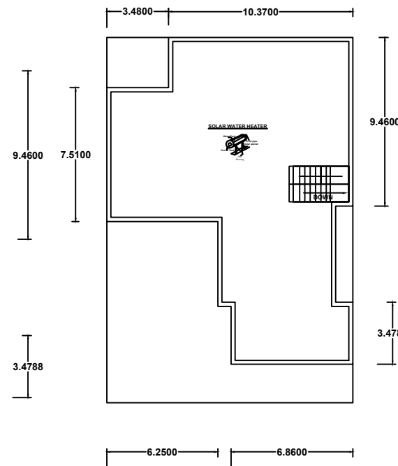
Open Terrace
