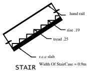
STAIR
