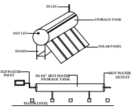
SOLAR HOT WATER SYSTEM DETAIL
