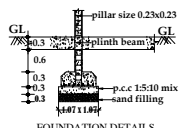
FOUNDATION DETAIL
