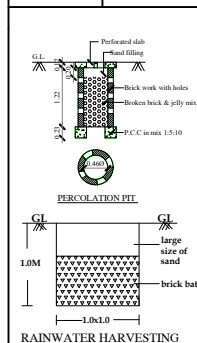
RAINWATER HARVESTING
