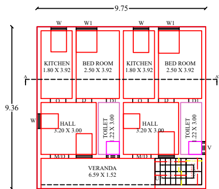
GROUND FLOOR PLAN (NORTH FACING)
