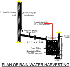
PLAN OF RAIN WATER HARVESTING
