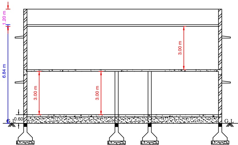
SECTION ON - A
