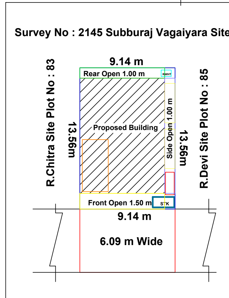
Site Plan
