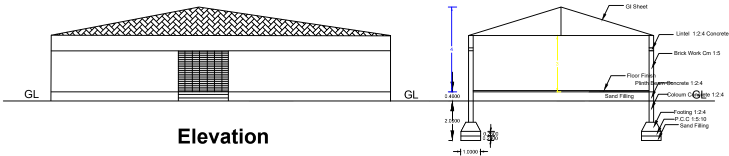
Section Section - AA
