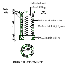
PERCOLATION PIT
