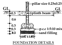
FOUNDATION DETAILS
