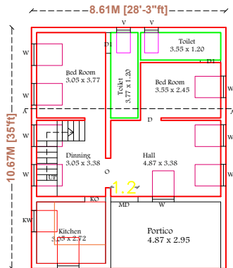
GROUND FLOOR PLAN (FACING EAST)
